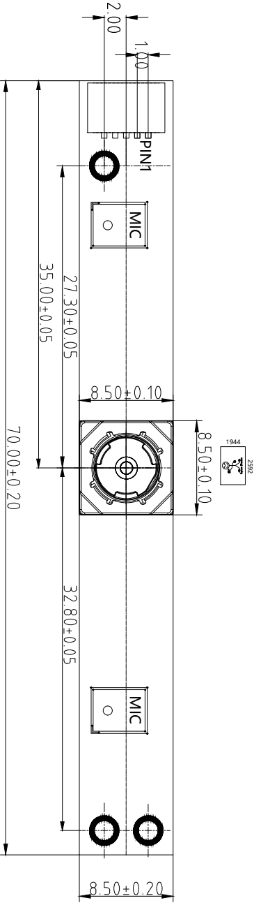
TOP VIEW
